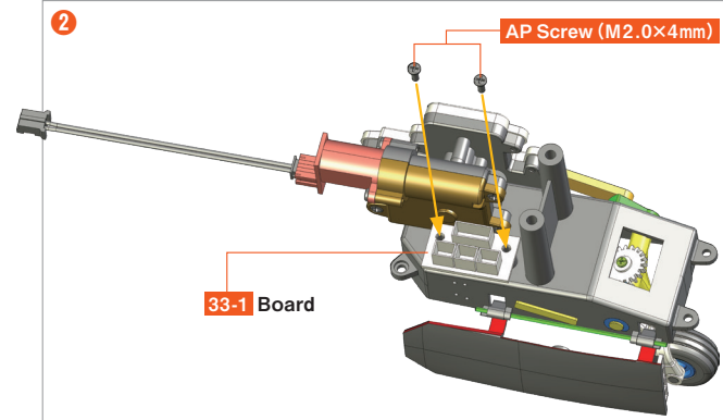
33-1 Board
